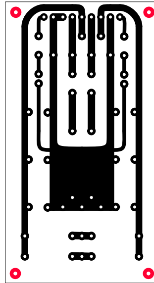
Trace mask
