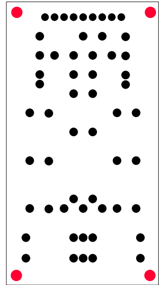
Solder mask
